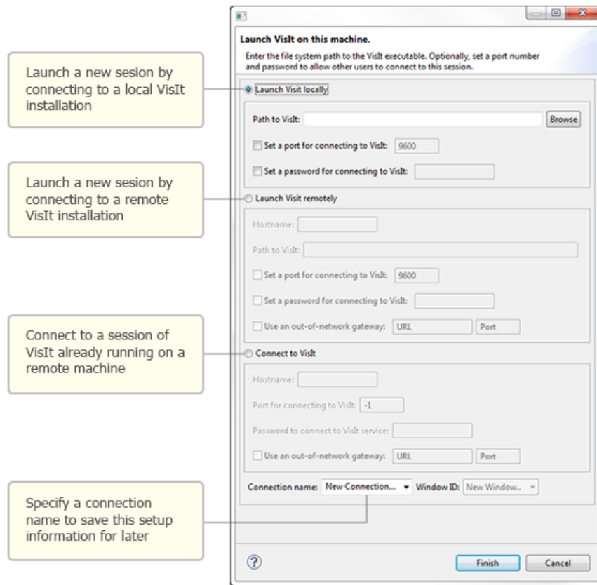
Figure 3.6: The VisIt connection wizard in ICE.
